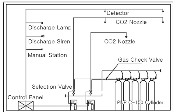
SYSTEM LAYOUT
