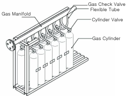
INSTALLATION FIGURE
